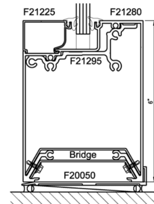
6" Sill Section
