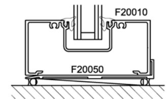
Sill Section
