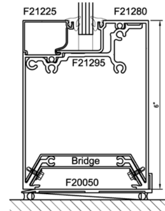
6" Sill Section
