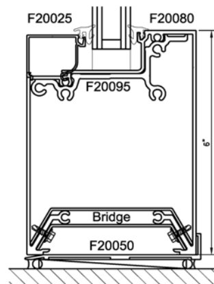
6" Sill Section
