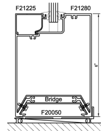
6" Sill Section
