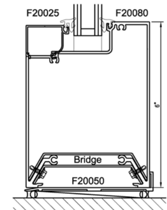
6" Sill Section
