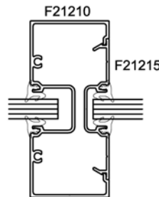
Screw Spline Vertical Mullion Section
