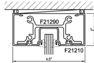
Head/Jamb Section
