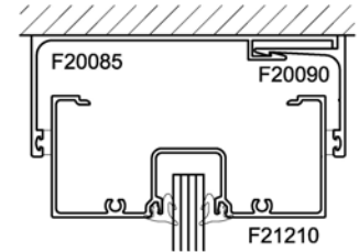
Head Receptor Section
