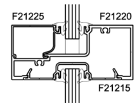
Intermediate Horizontal Section
