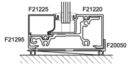
Sill Section
