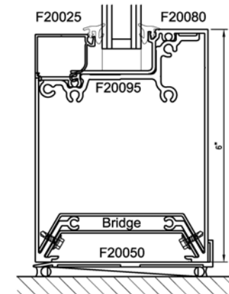
6" Sill Section
