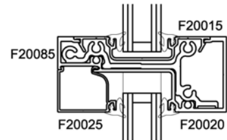
Intermediate Horizontal Section
