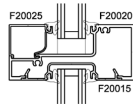
Intermediate Horizontal Section
