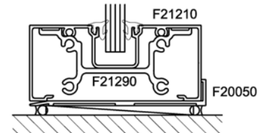
Sill Section
