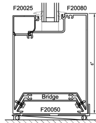
6" Sill Section
