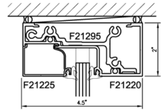
Head/Jamb Section
