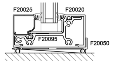
Sill Section
