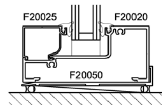
Sill Section
