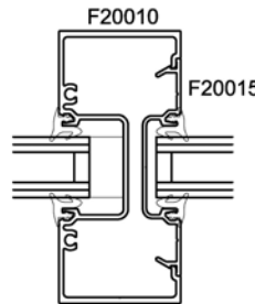
Screw Spline Vertical Mullion Section
