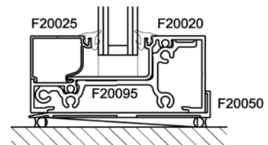
Sill Section
