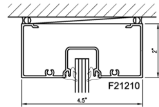
Head/Jamb Section
