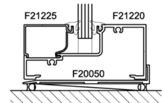
Sill Section
