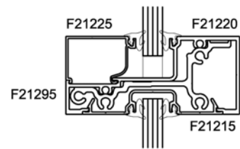
Intermediate Horizontal Section
