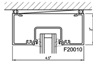
Head/Jamb Section
